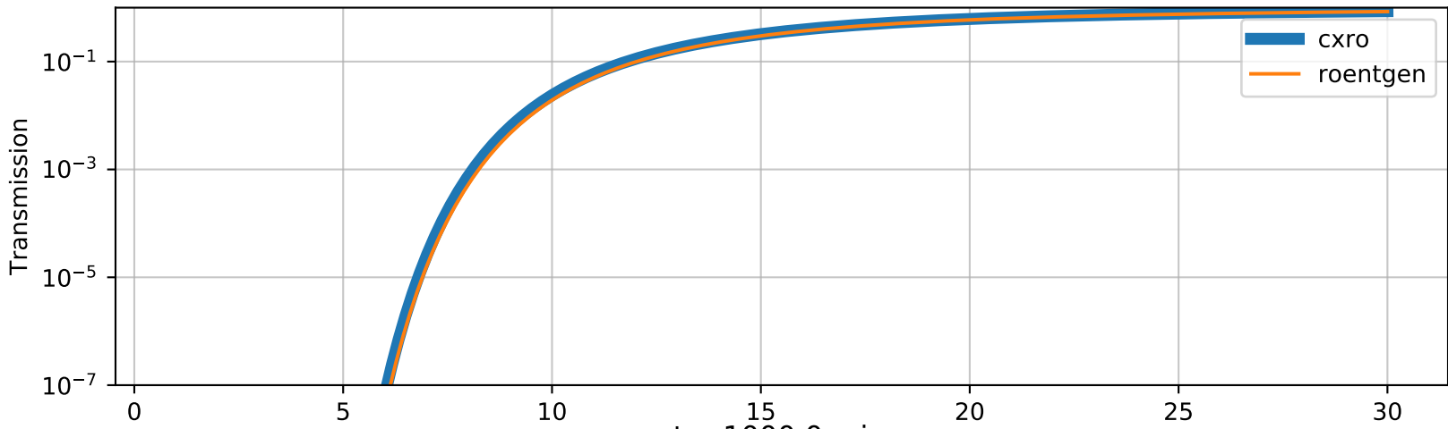
water 1000.0 micron
