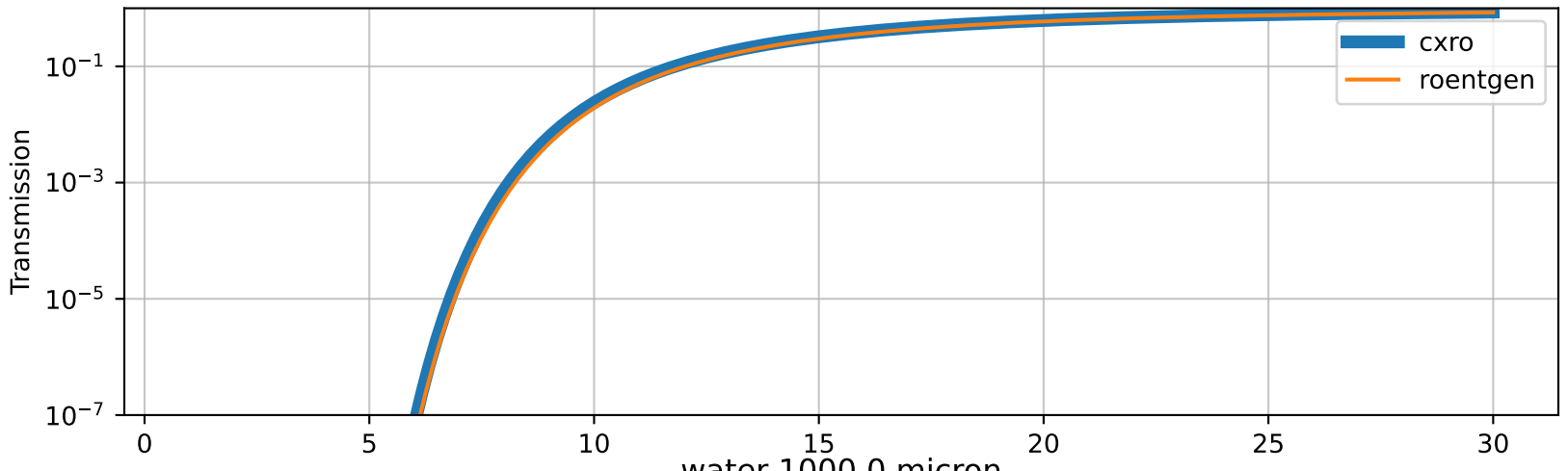
water 1000.0 micron
