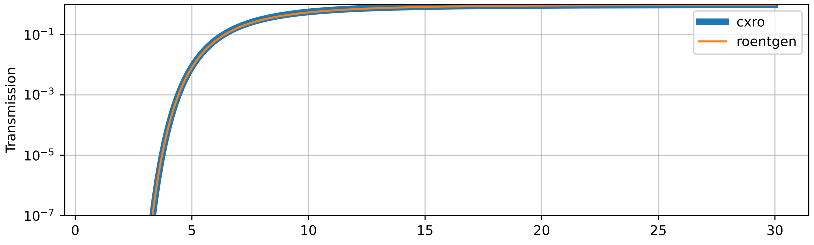
air 1.0 m
